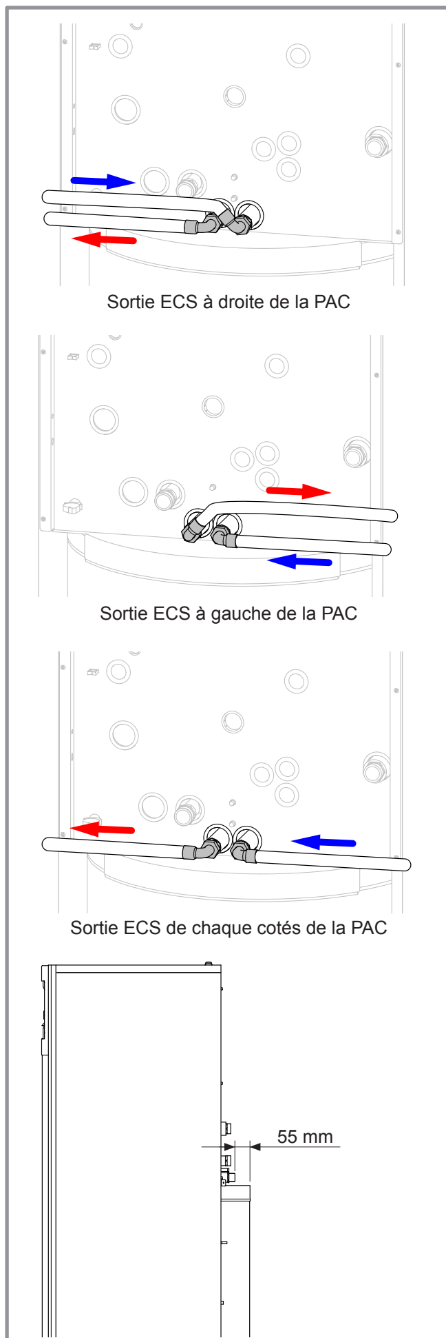
figure 26 - Sorties circuit ECS
